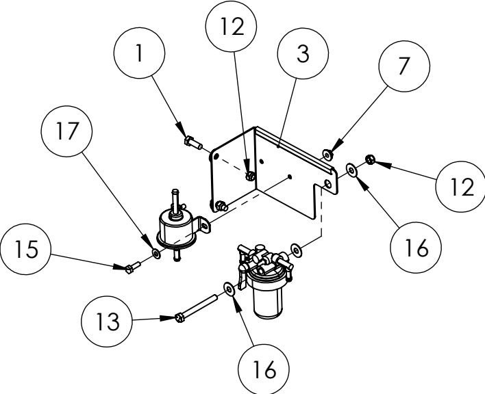
* FUEL PUMP & WATER SEPARATOR MOUNTING*
