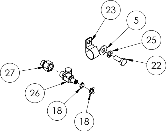
* DRAIN VALVE & HOSE CLAMP*
